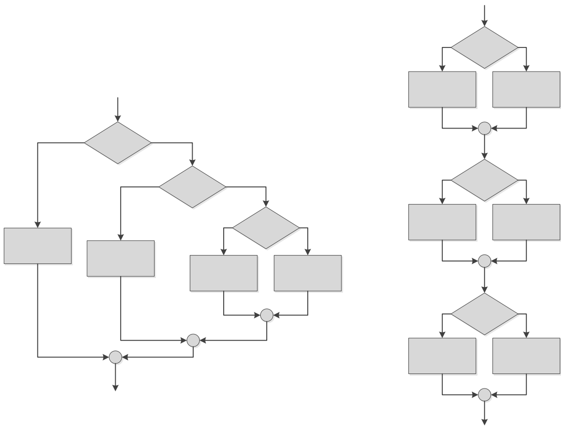
Figure 5.6 The structure of the if statements in a program such as Listing 5.15 ( restyleddigittoword.cpp ) (left) vs. those in a program like Listing 5.9 ( binaryconversion.cpp ) (right)
