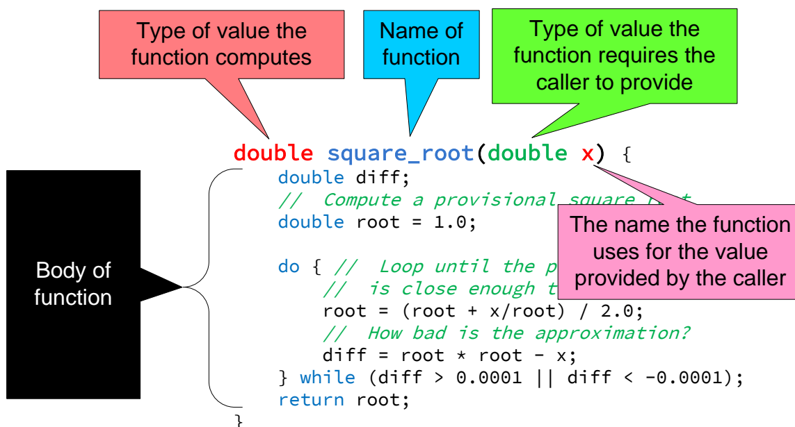
Figure 9.1 Function definition dissection
