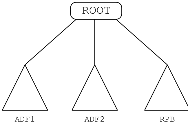
Figure 6.1: Example of program structure with two automatically-defined functions (ADF1 and ADF2) and one result-producing branch (RPB).
